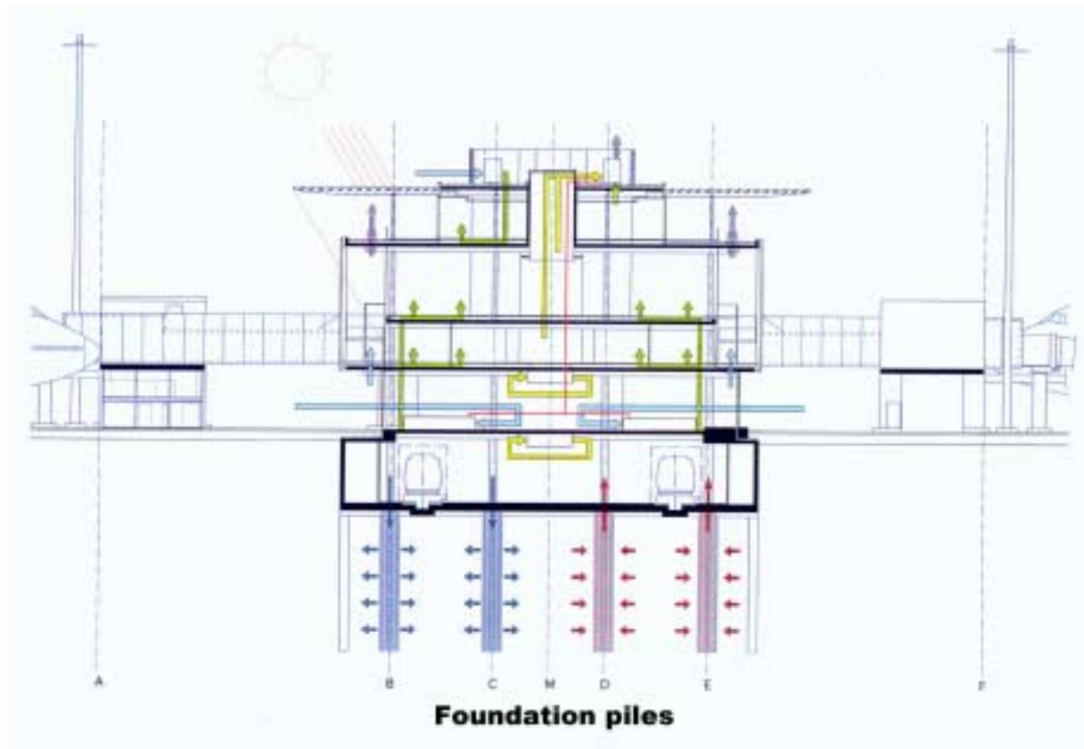
Fig. 1.1 Cross section of Dock Midfield.
