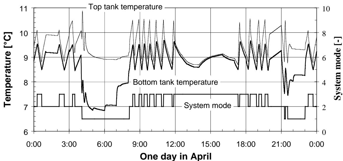
Fig. 5.13 The system dynamic is simulated with a time-step of 45 sec. The two graphs illustrate the response of the system to the heating and cooling demand. The fluid temperatures are simulated in the cold storage.
