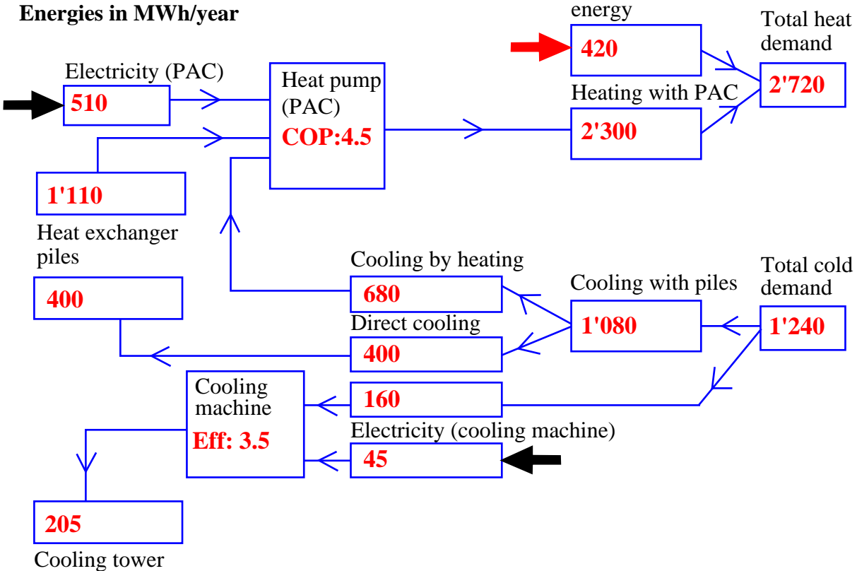
Fig. 4.2 Annual energy fluxes through the pile system, average values for the first 10 years of operation (simulated with PILESIM).
