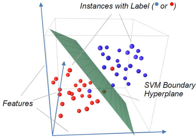
Fig. 1: Example of a boundary hyperplane identified by SVM.
