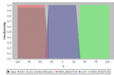
Fig. 13: Membership function: defuzzification of EAX error
